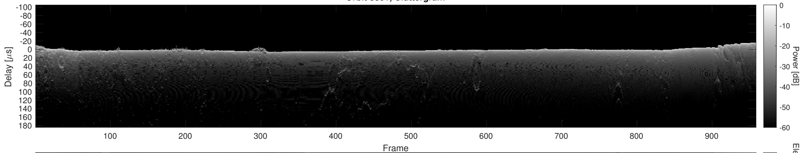
Orbit 3861, Cluttergram
