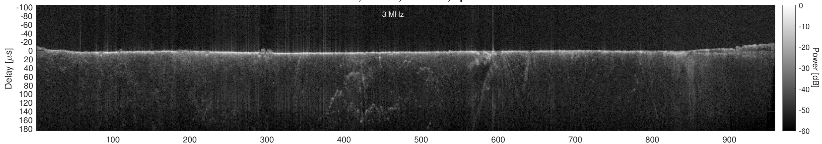
Orbit 3861, Cluttergram
