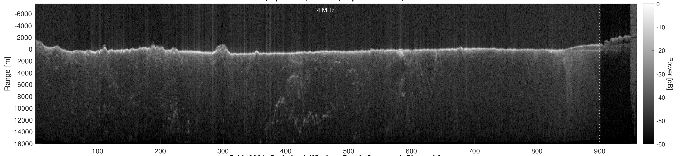
Orbit 3861, Optimized, Window, Depth-Corrected, Channel 2
