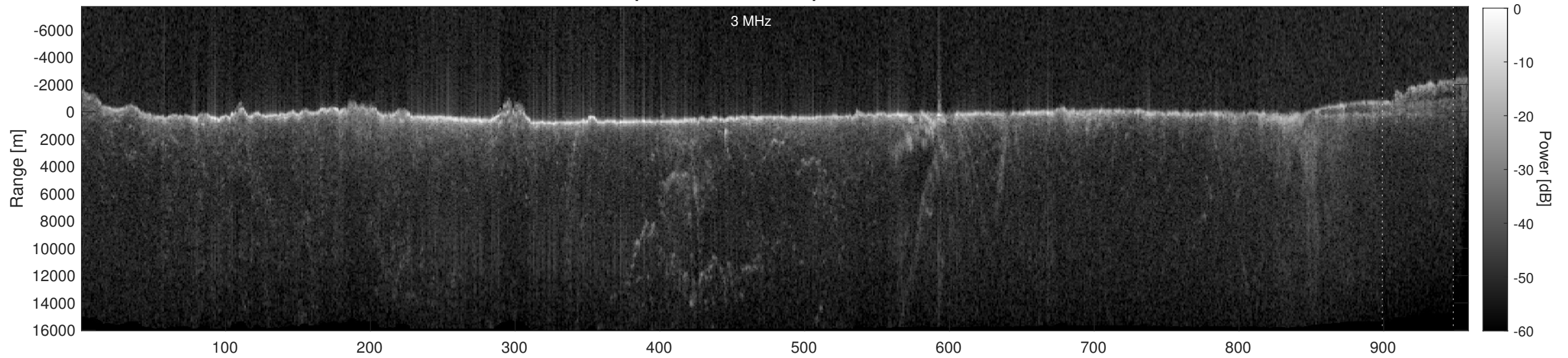
Orbit 3861, Depth-Corrected Cluttergram
