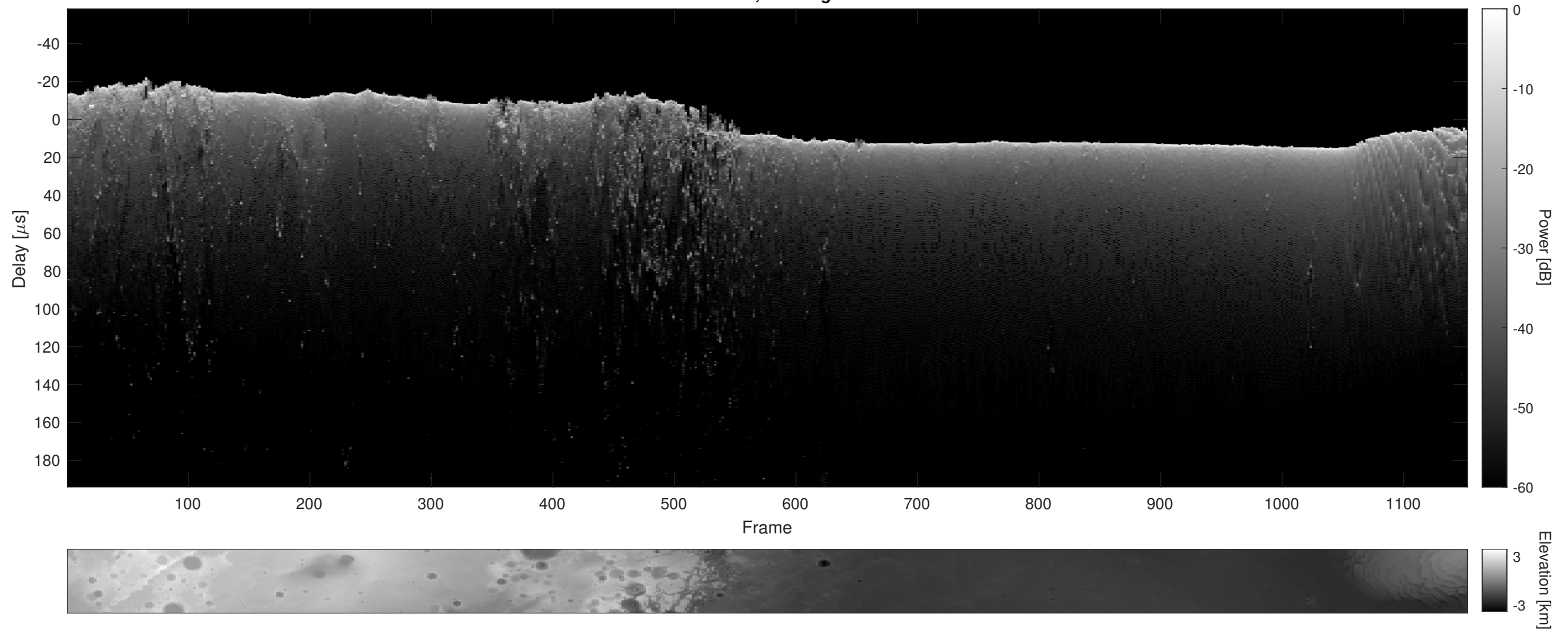
Orbit 3862, Cluttergram
