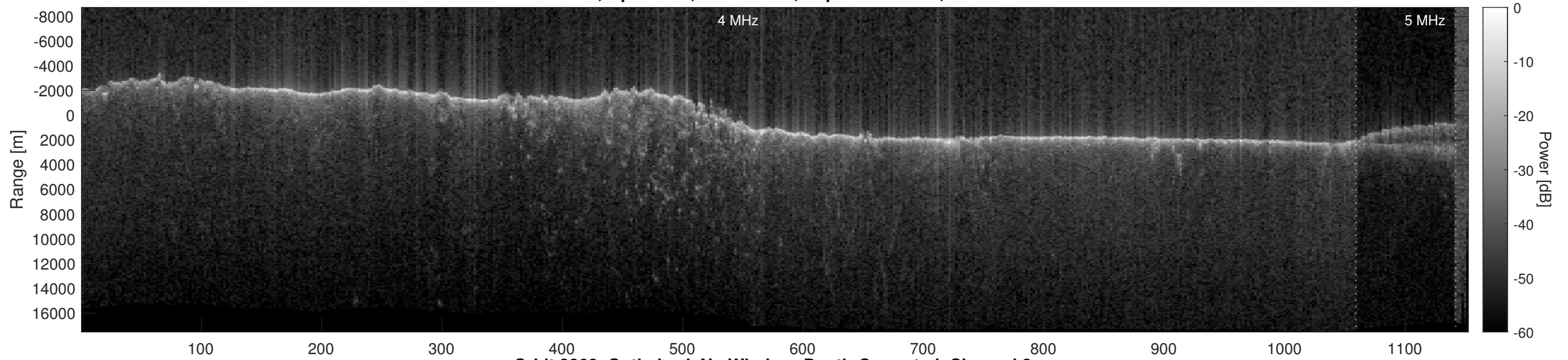
Orbit 3862, Optimized, No Window, Depth-Corrected, Channel 2
