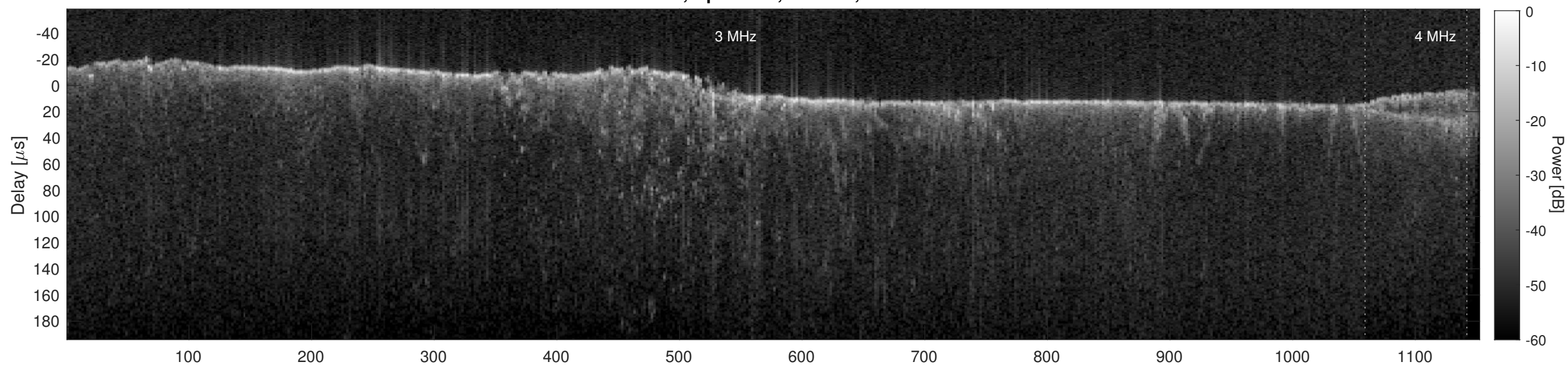
Orbit 3862, Cluttergram
