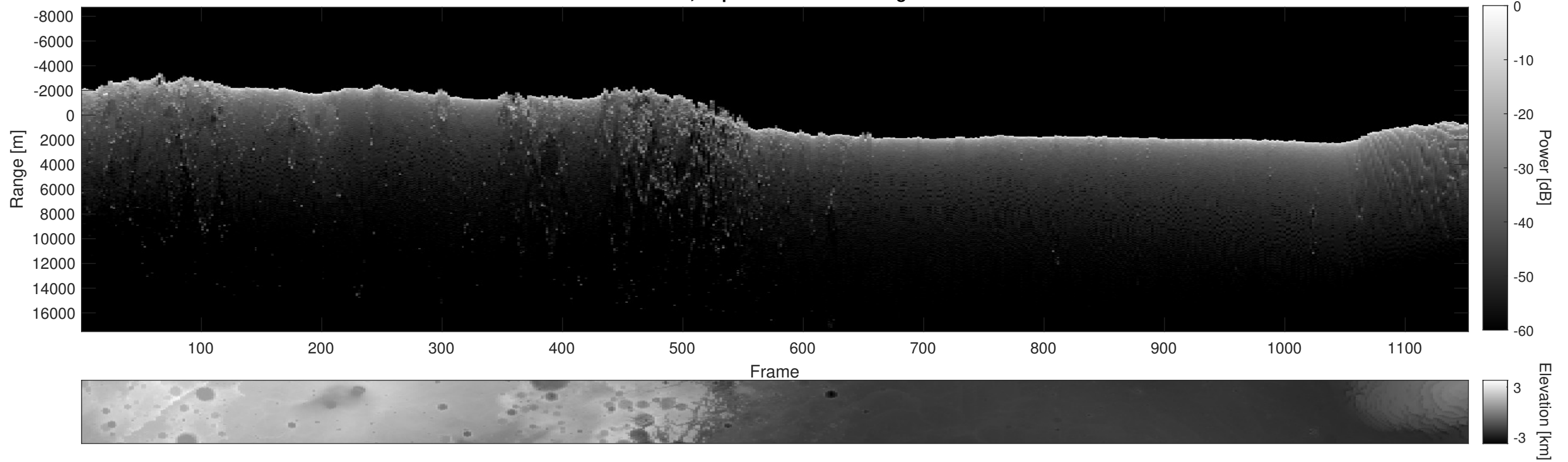
Orbit 3862, Depth-Corrected Cluttergram
