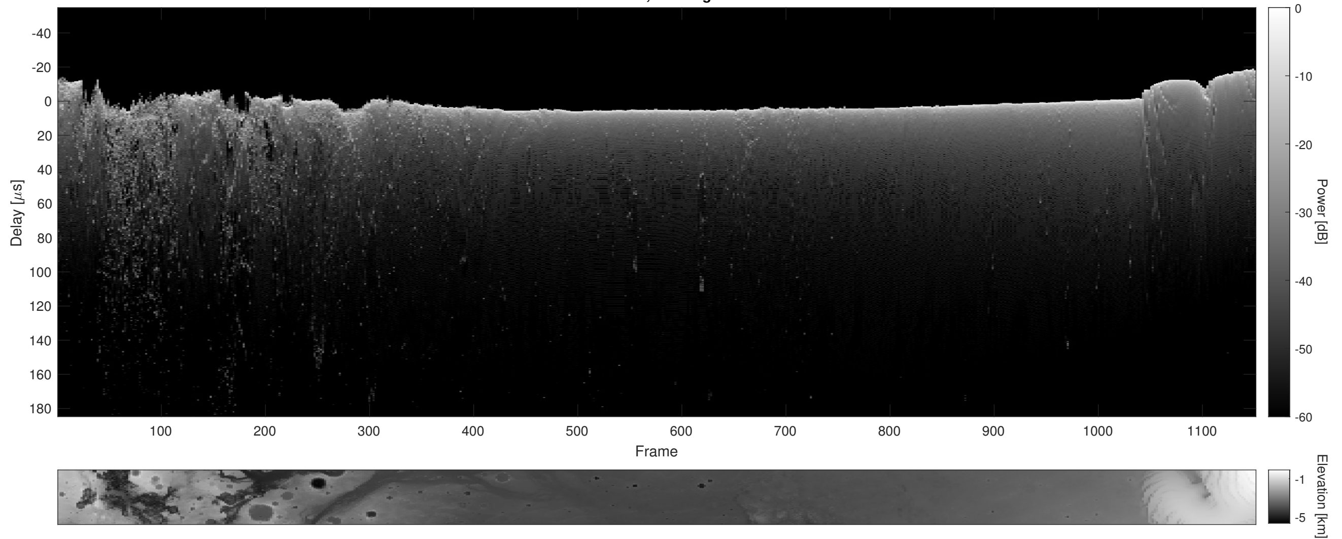
Orbit 3863, Cluttergram
