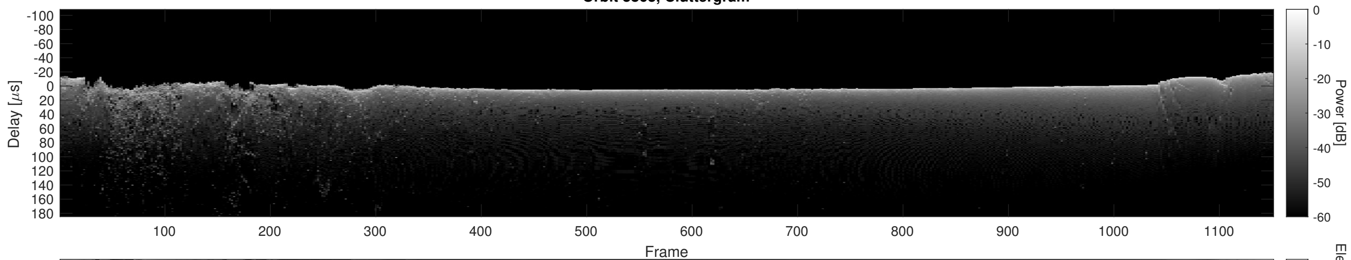
Orbit 3863, Cluttergram
