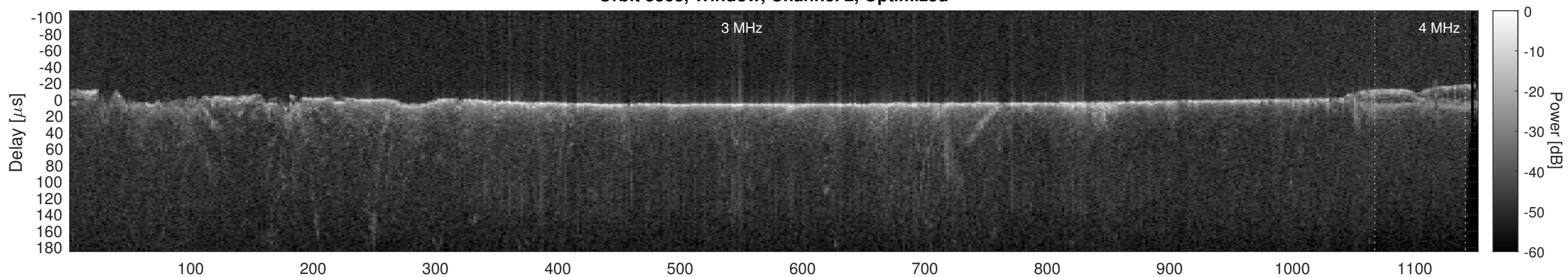
Orbit 3863, Cluttergram
