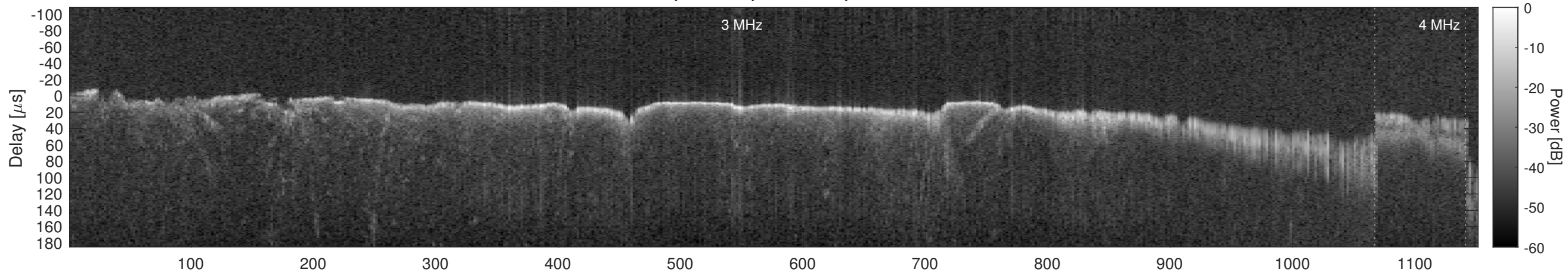
Orbit 3863, Window, Channel 2, Chapman
