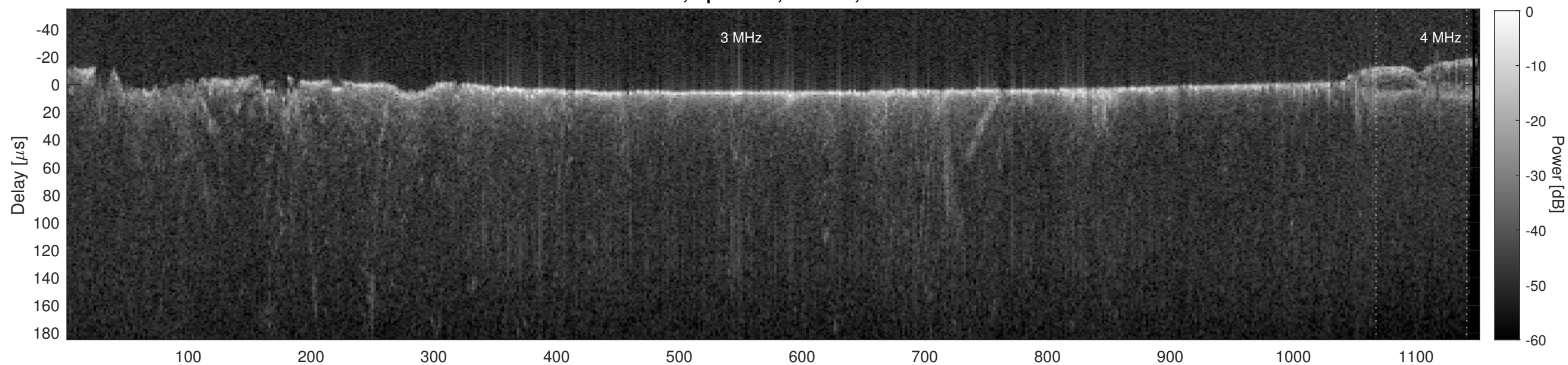
Orbit 3863, Cluttergram
