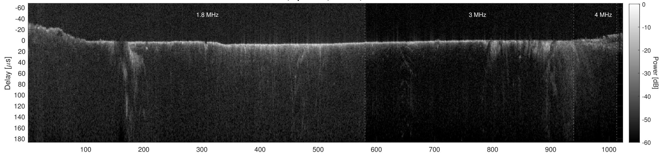
Orbit 3865, Cluttergram
