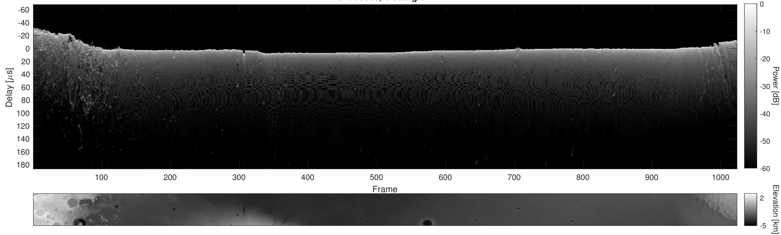
Orbit 3865, Cluttergram
