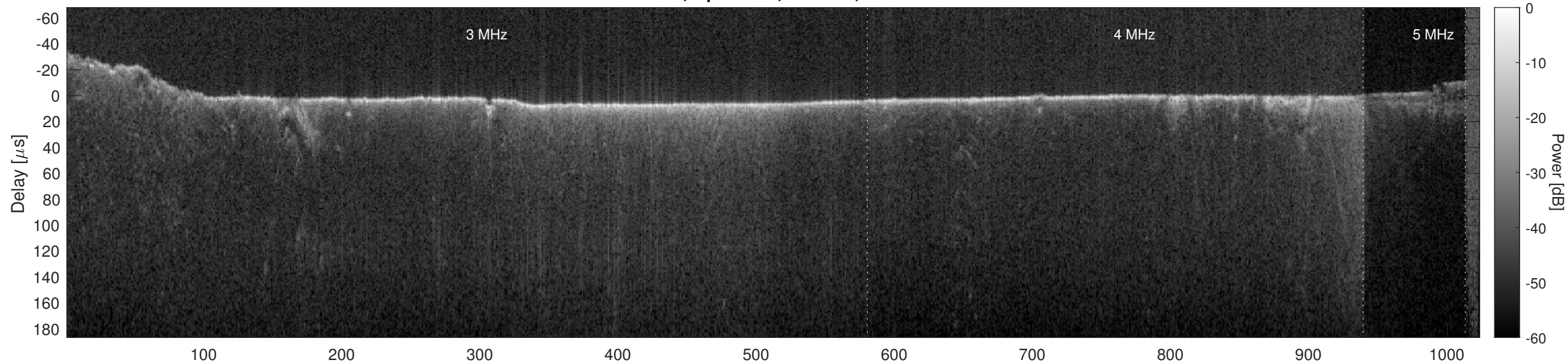
Orbit 3865, Optimized, Window, Channel 2
