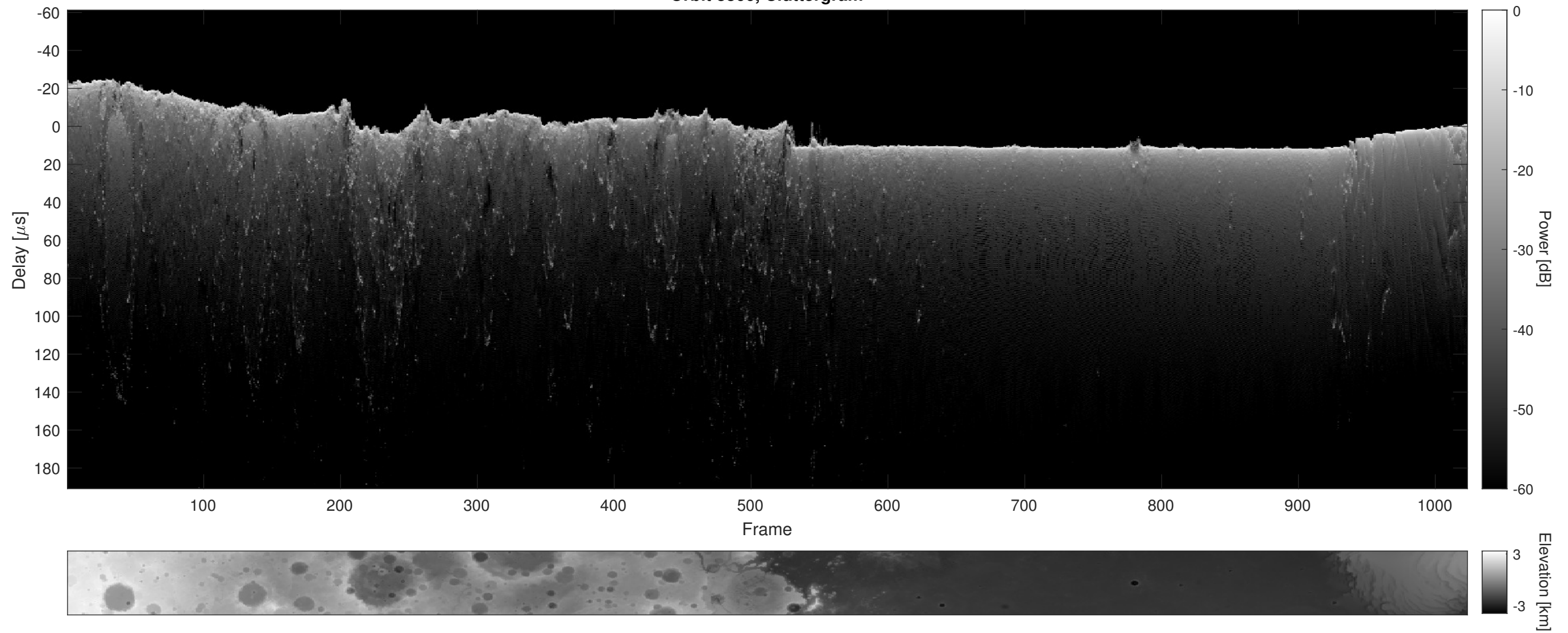
Orbit 3866, Cluttergram
