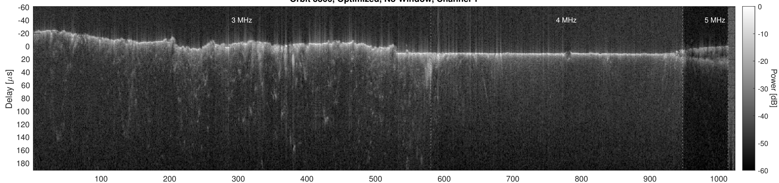
Orbit 3866, Optimized, No Window, Channel 2
