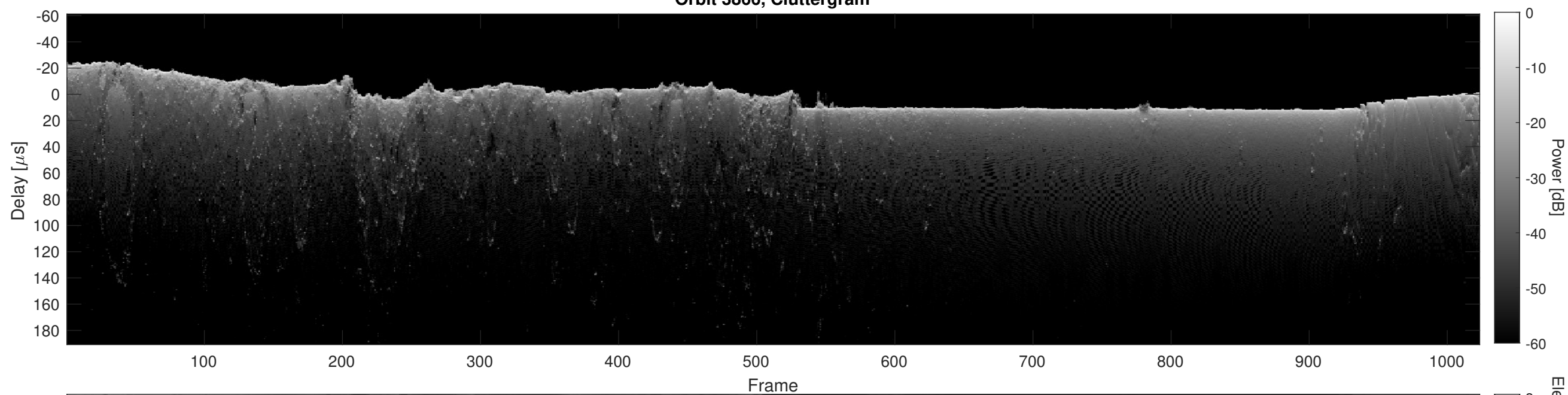
Orbit 3866, Cluttergram
