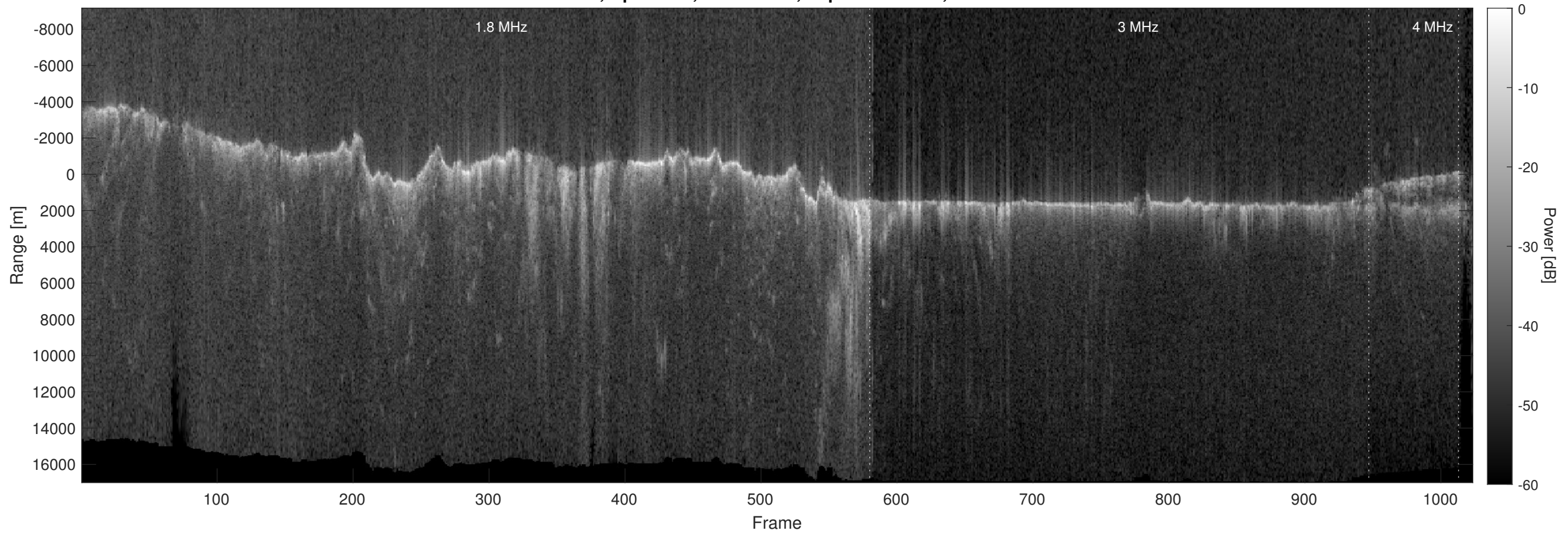
Orbit 3866, Optimized, No Window, Depth-Corrected, Channel 2
