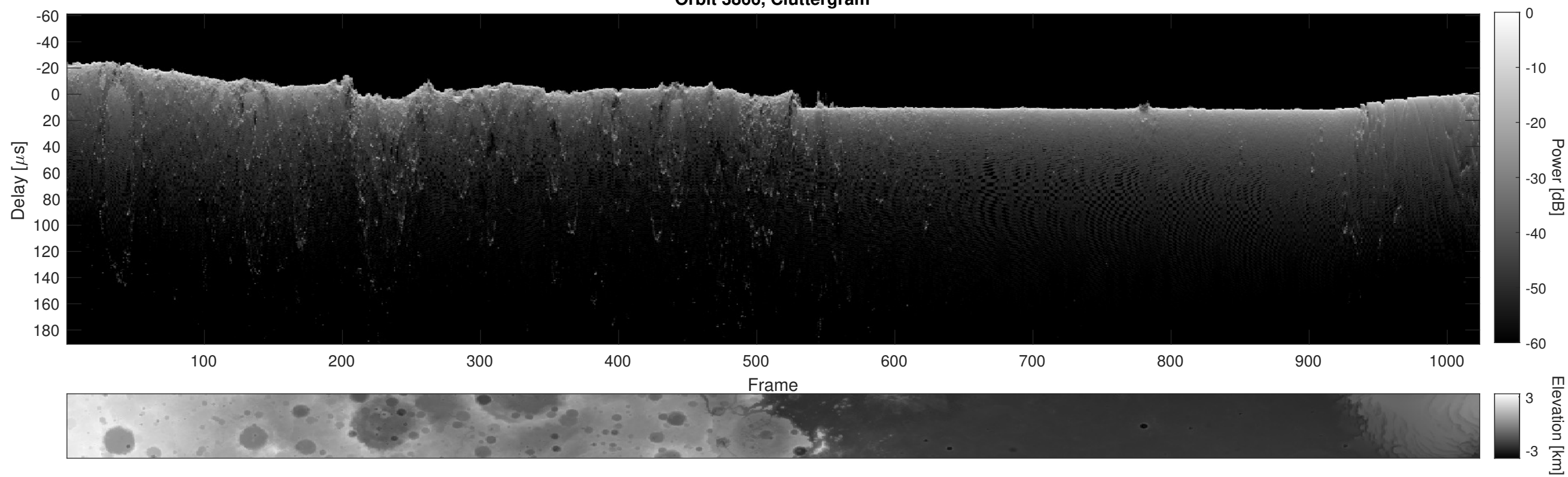
Orbit 3866, Cluttergram
