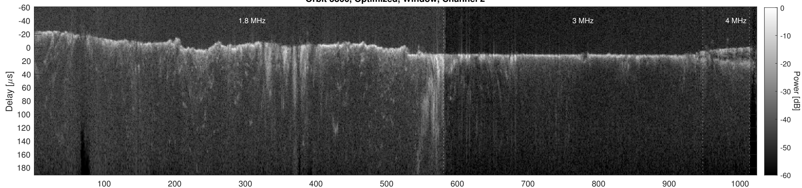
Orbit 3866, Cluttergram
