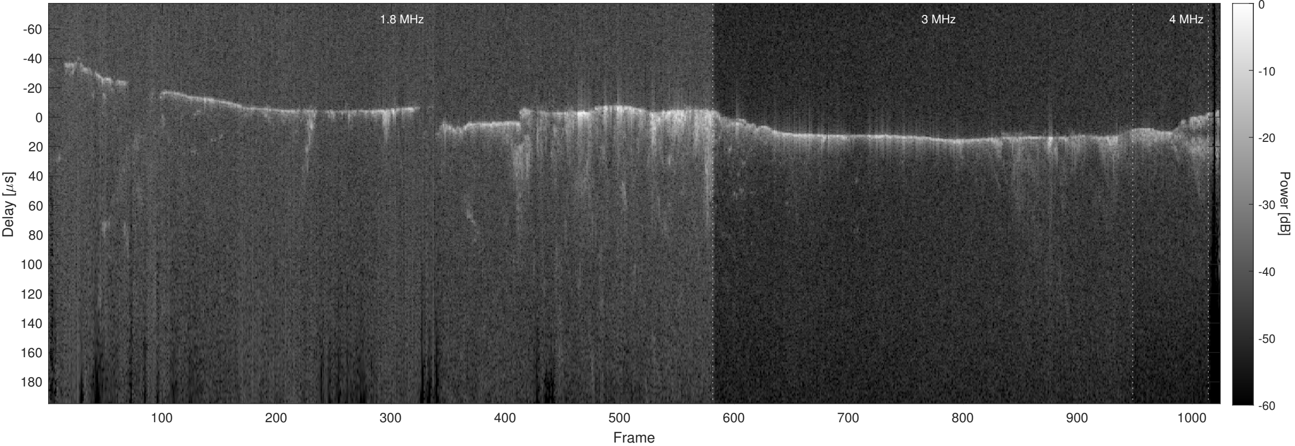
Orbit 3867, Optimized, No Window, Channel 2
