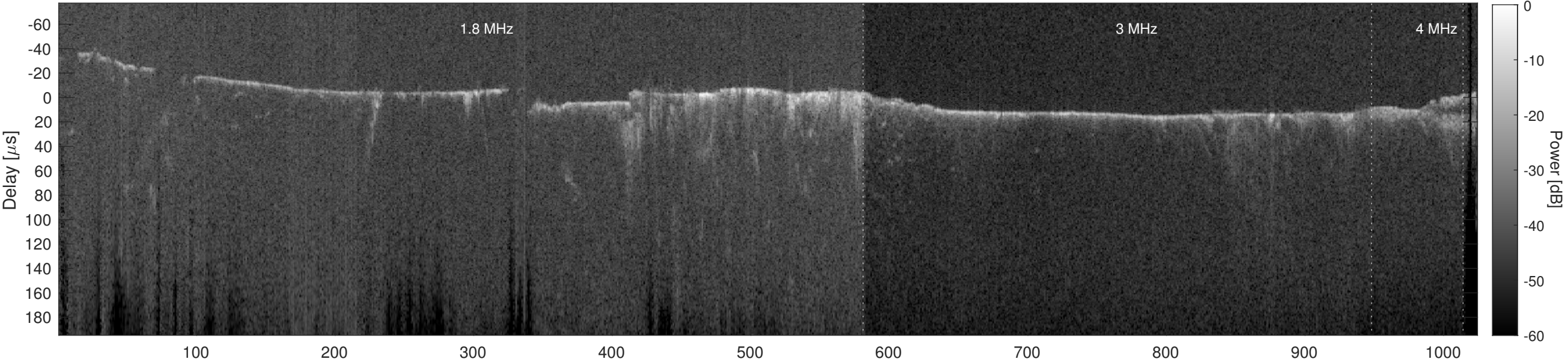
Orbit 3867, Cluttergram
