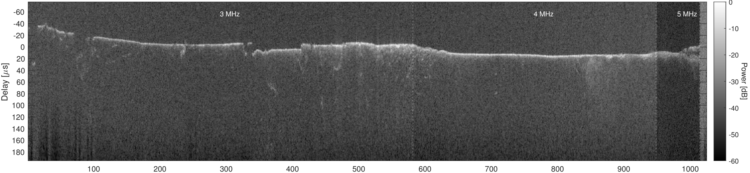
Orbit 3867, Optimized, Window, Channel 2
