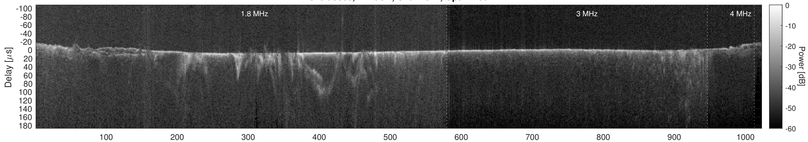
Orbit 3868, Cluttergram
