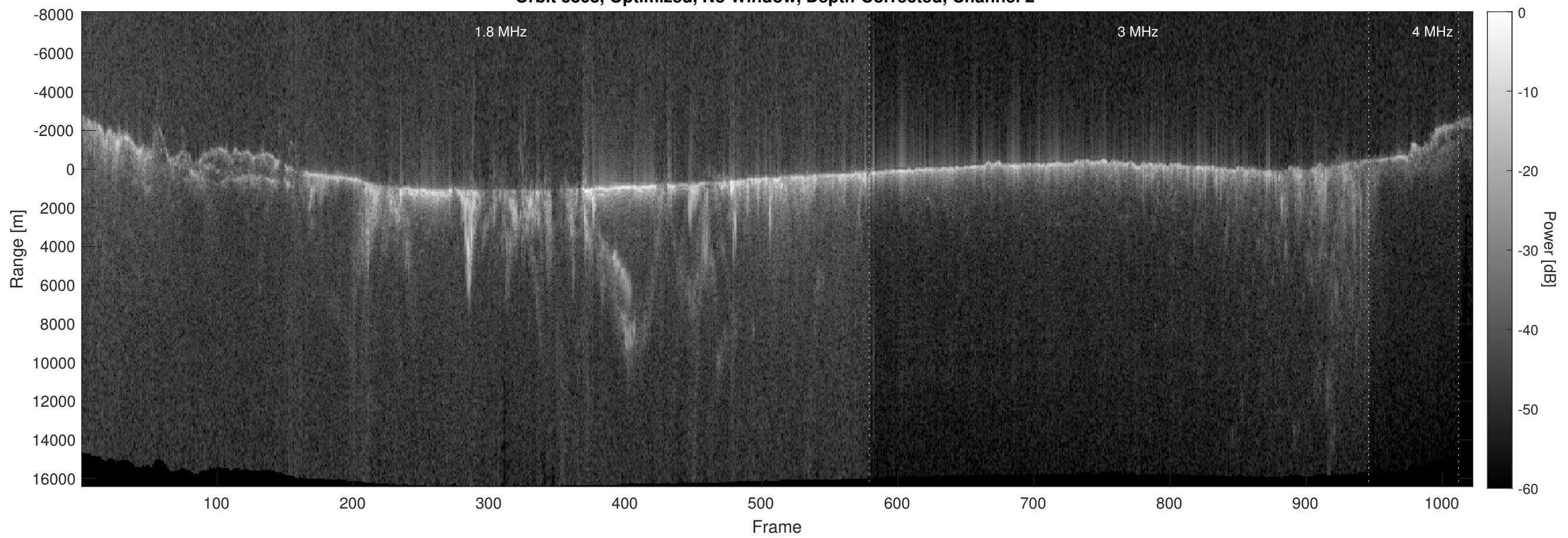
Orbit 3868, Optimized, No Window, Depth-Corrected, Channel 2
