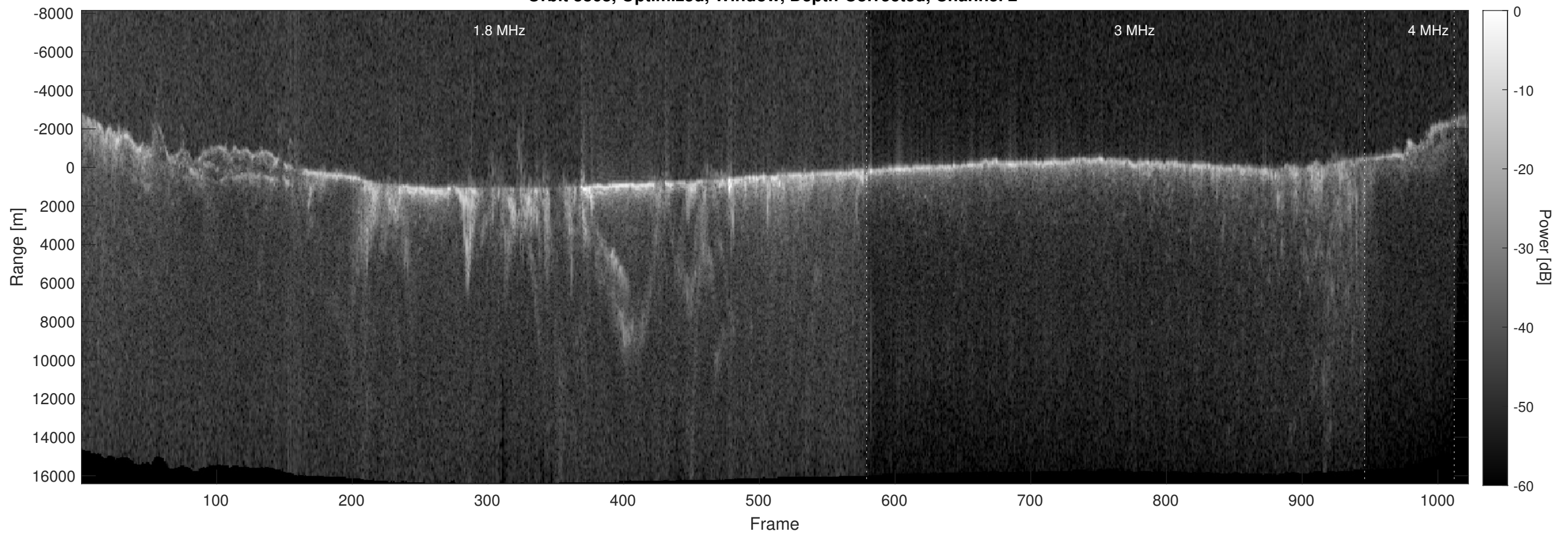
Orbit 3868, Optimized, Window, Depth-Corrected, Channel 2
