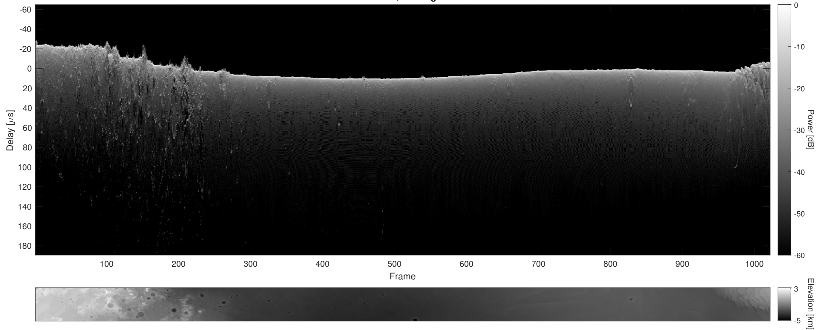
Orbit 3869, Cluttergram
