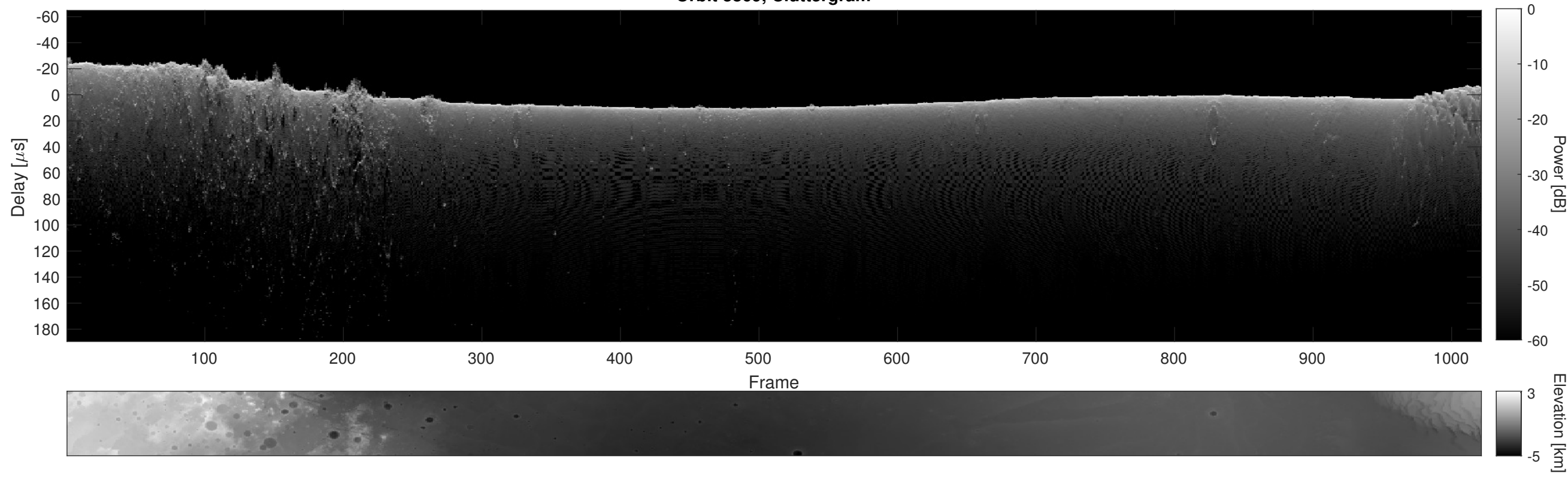
Orbit 3869, Cluttergram
