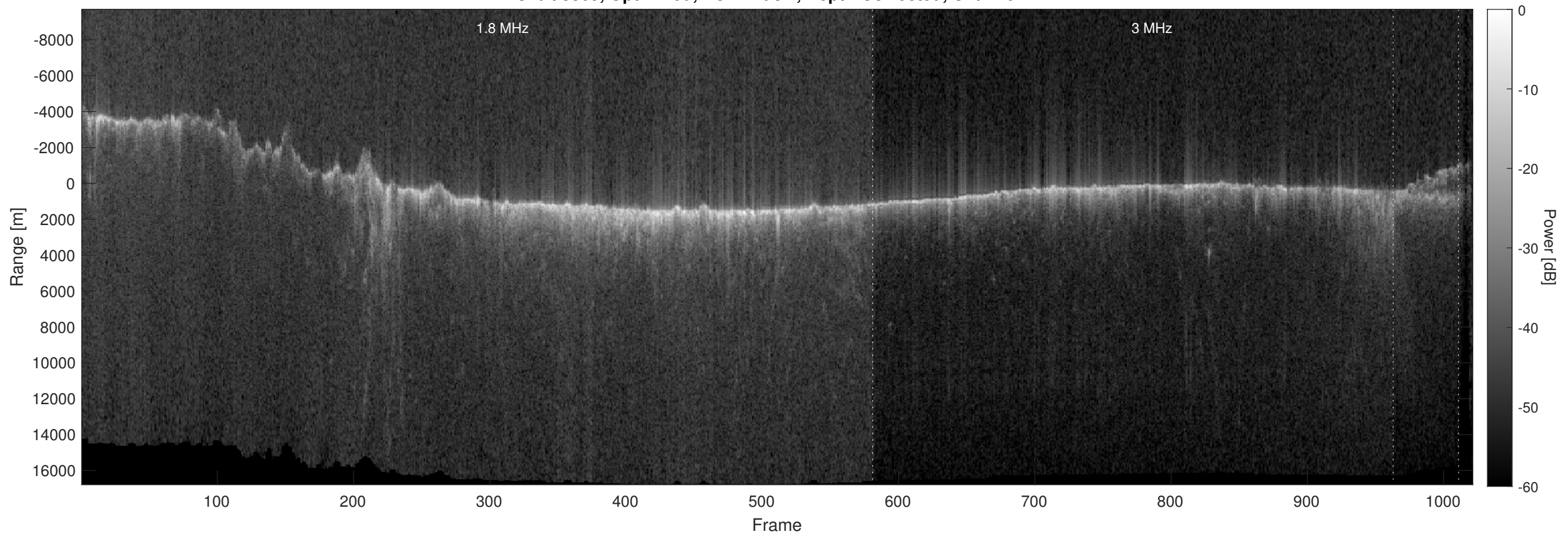
Orbit 3869, Optimized, No Window, Depth-Corrected, Channel 2
