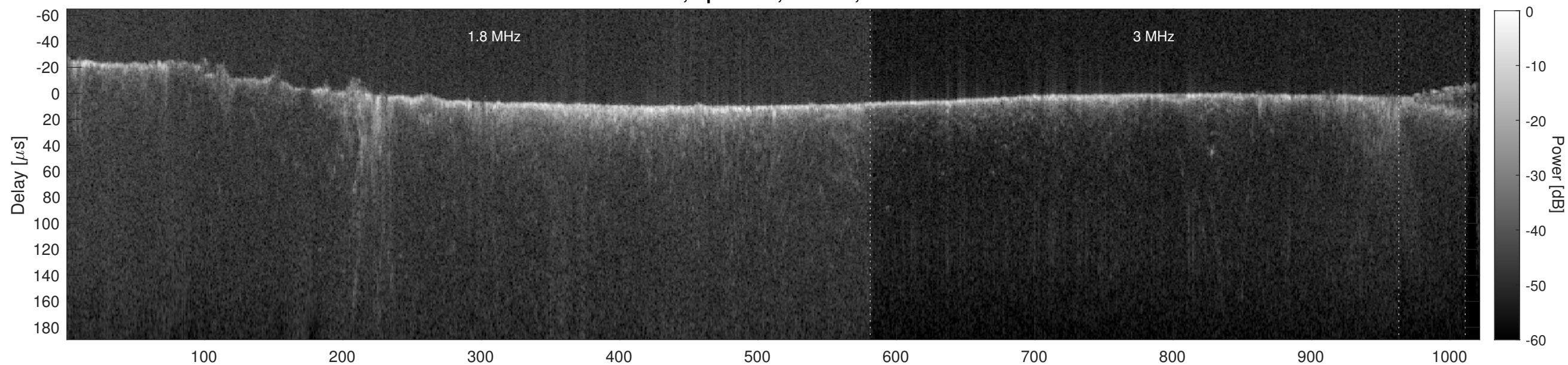
Orbit 3869, Cluttergram
