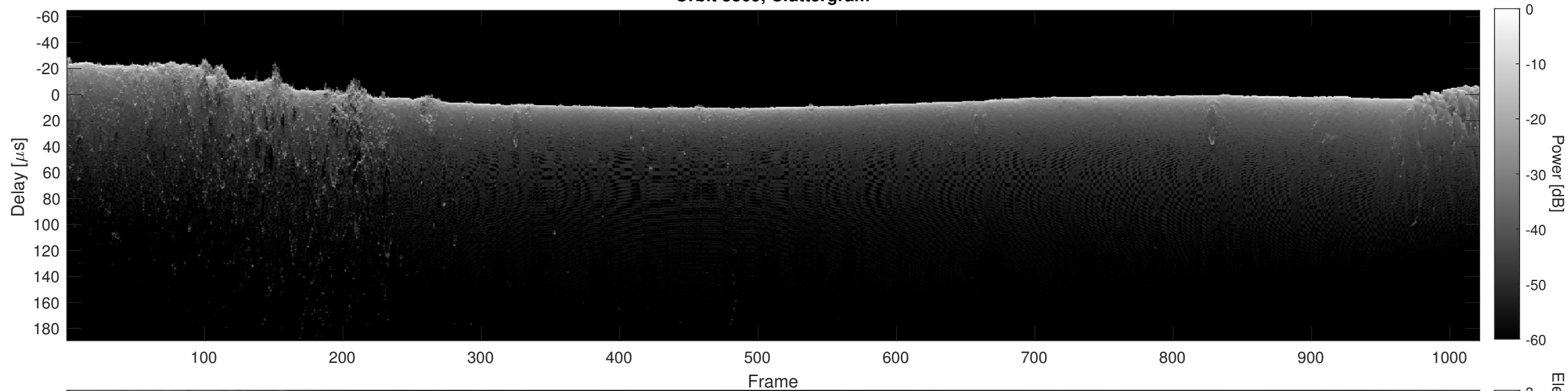
Orbit 3869, Cluttergram
