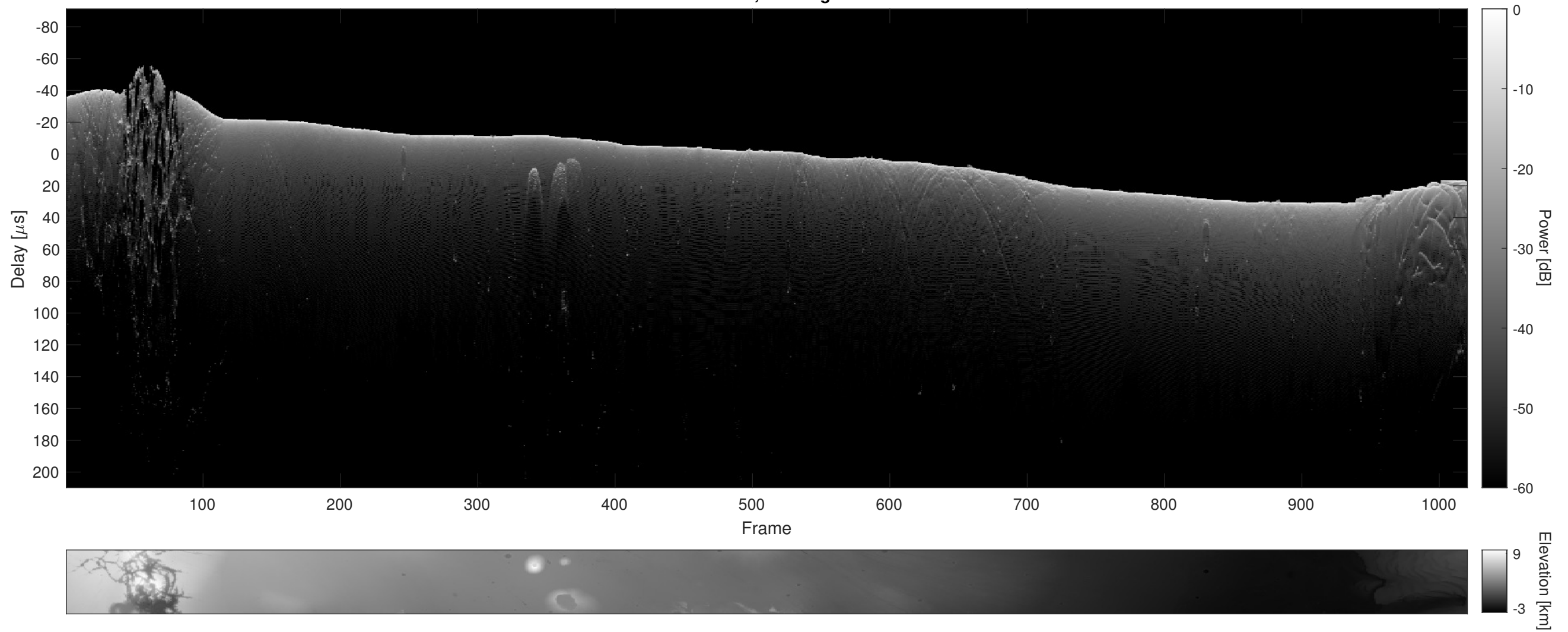
Orbit 3871, Cluttergram
