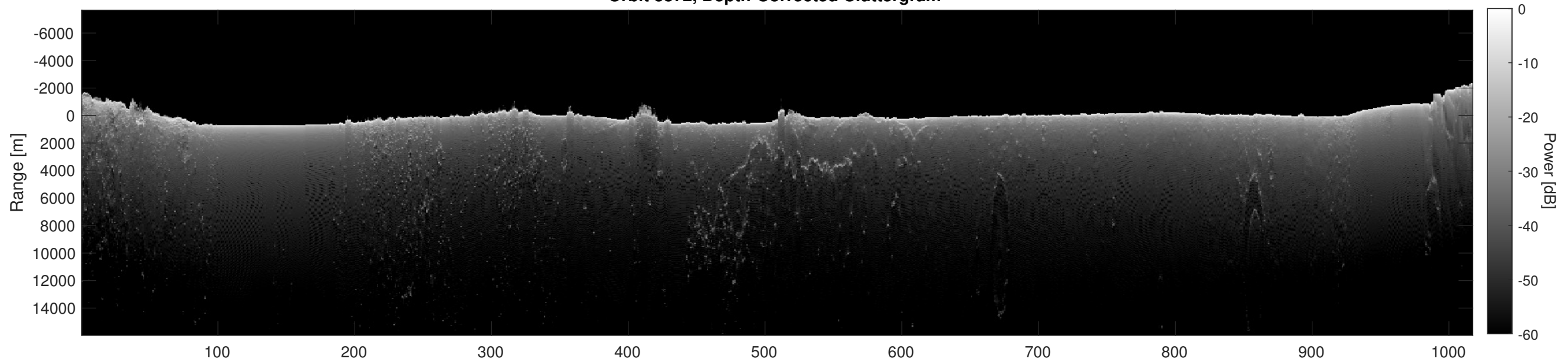
Orbit 3872, Depth-Corrected Cluttergram
