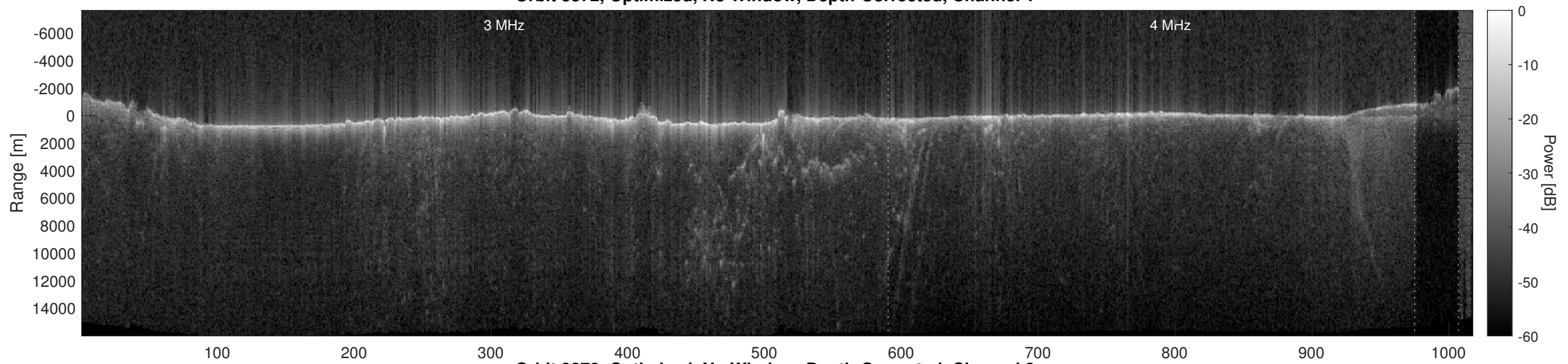
Orbit 3872, Optimized, No Window, Depth-Corrected, Channel 2
