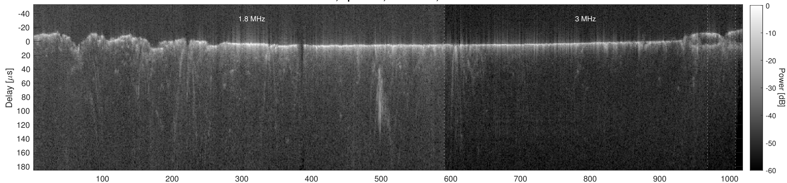
Orbit 3874, Cluttergram
