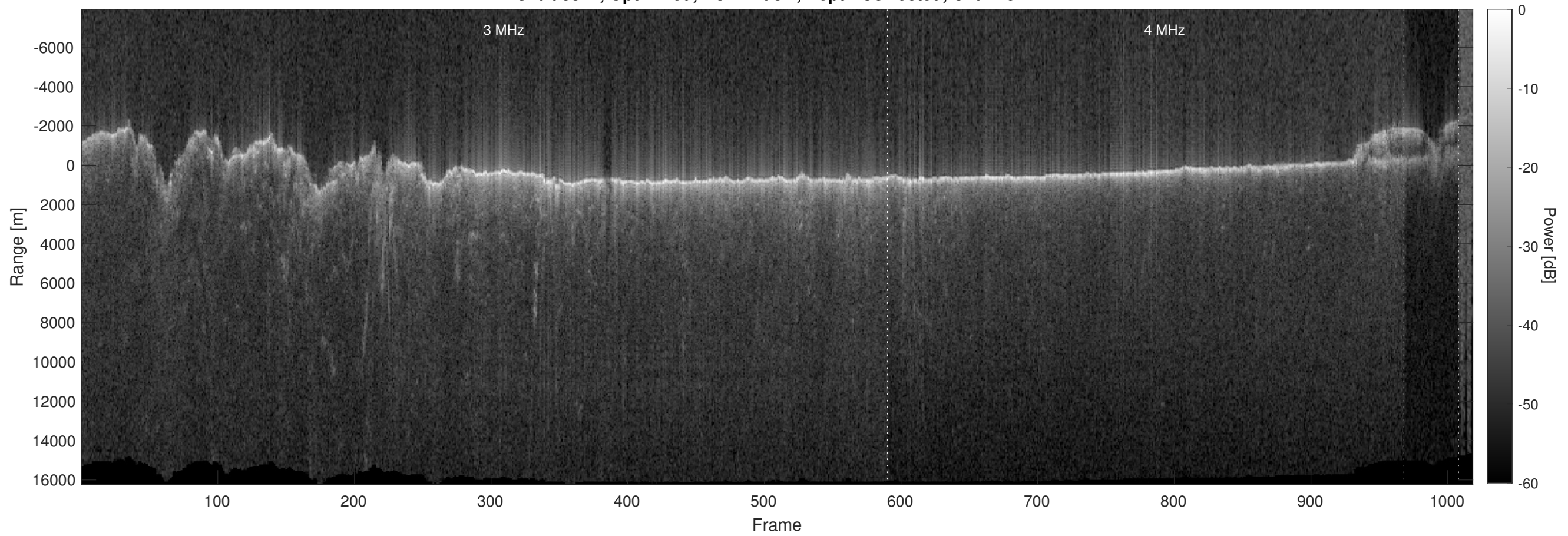
Orbit 3874, Optimized, No Window, Depth-Corrected, Channel 2
