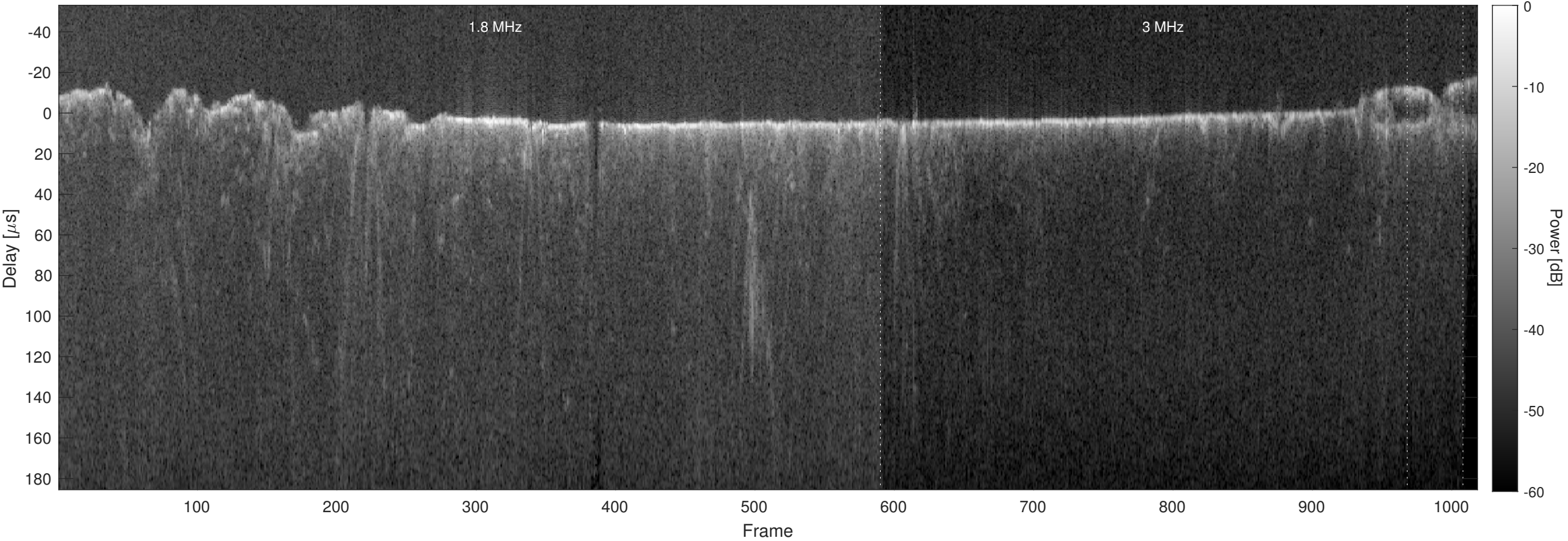
Orbit 3874, Optimized, Window, Channel 2
