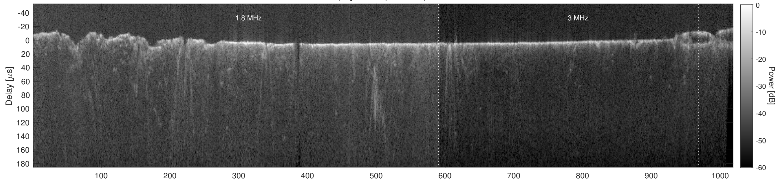
Orbit 3874, Cluttergram
