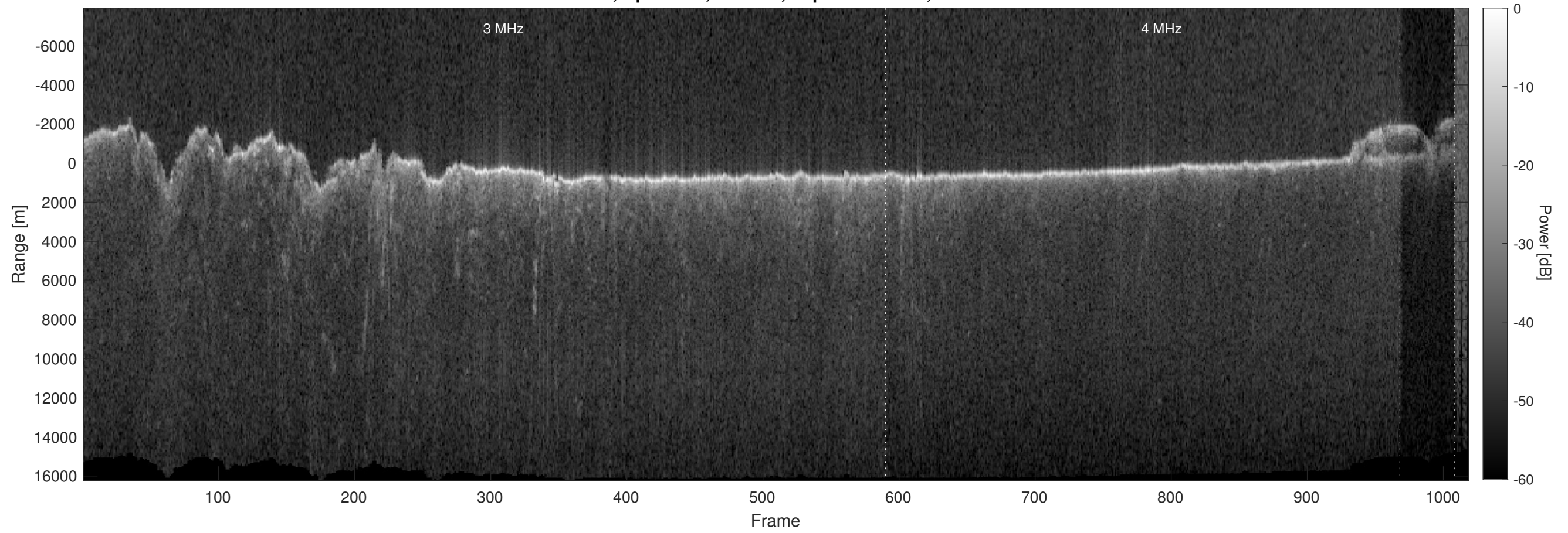
Orbit 3874, Optimized, Window, Depth-Corrected, Channel 2
