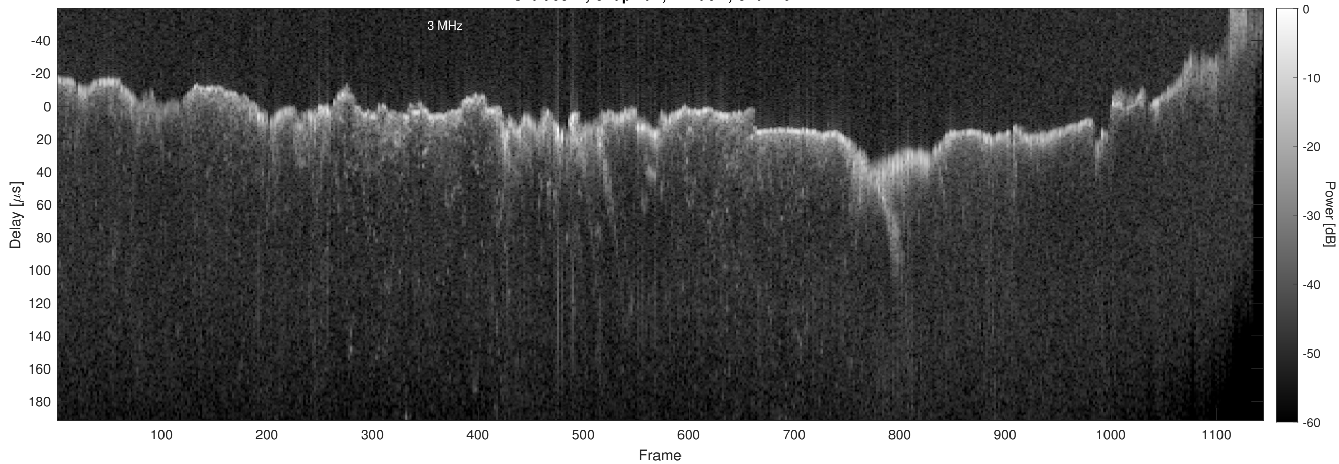
Orbit 3877, Chapman, Window, Channel 2
