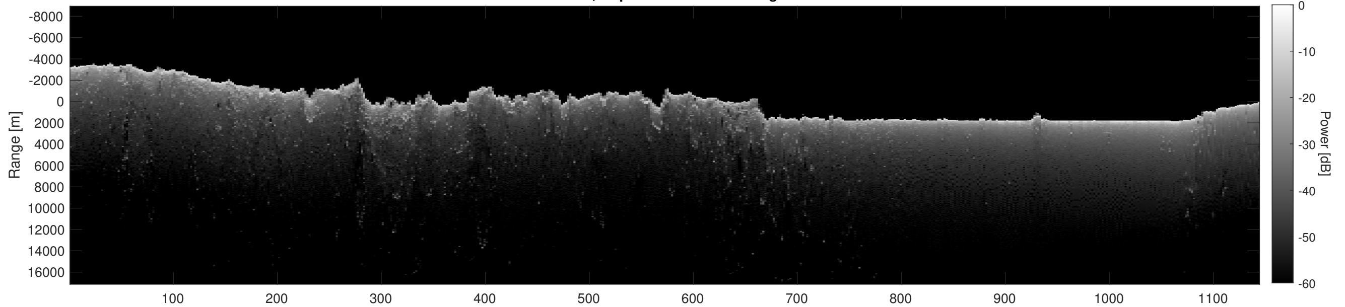
Orbit 3877, Depth-Corrected Cluttergram
