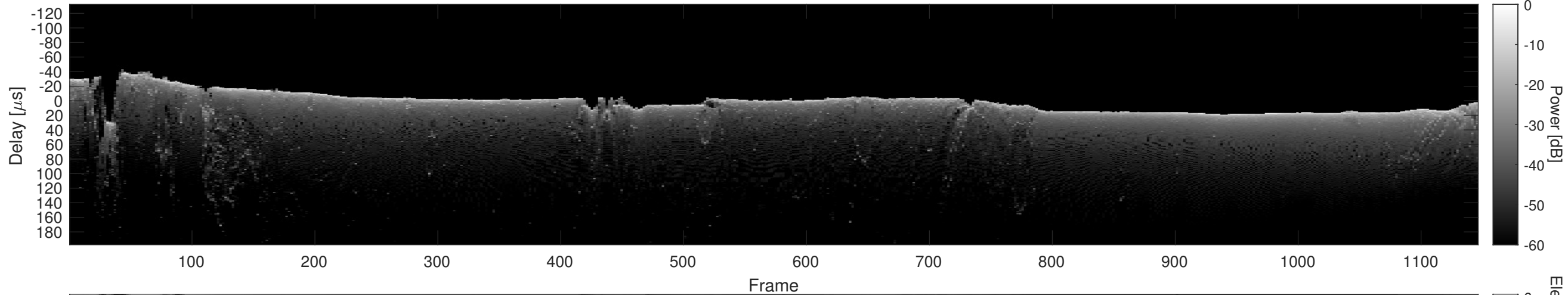
Orbit 3878, Cluttergram
