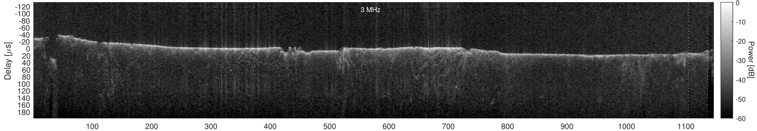
Orbit 3878, Cluttergram
