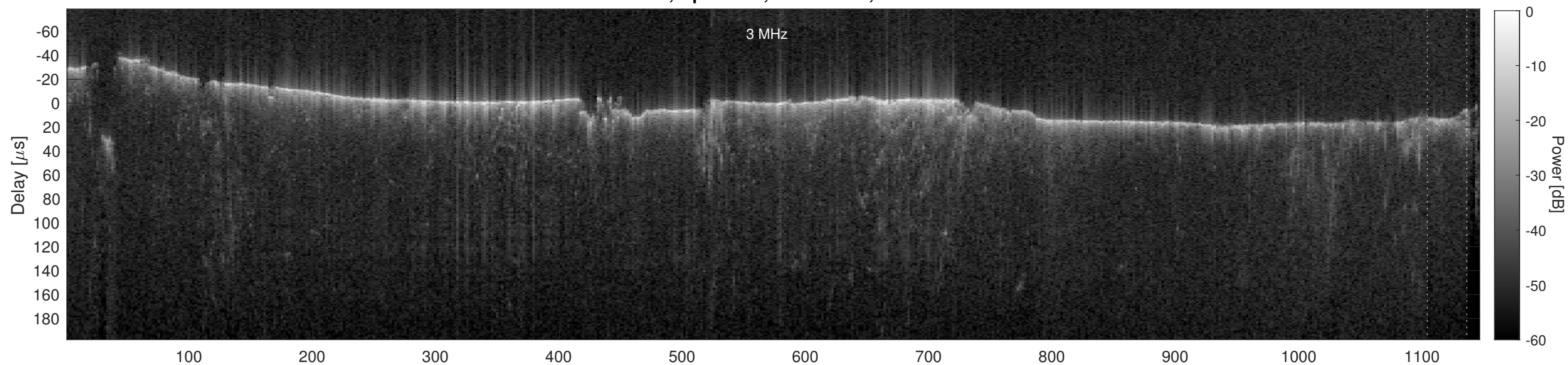
Orbit 3878, Cluttergram
