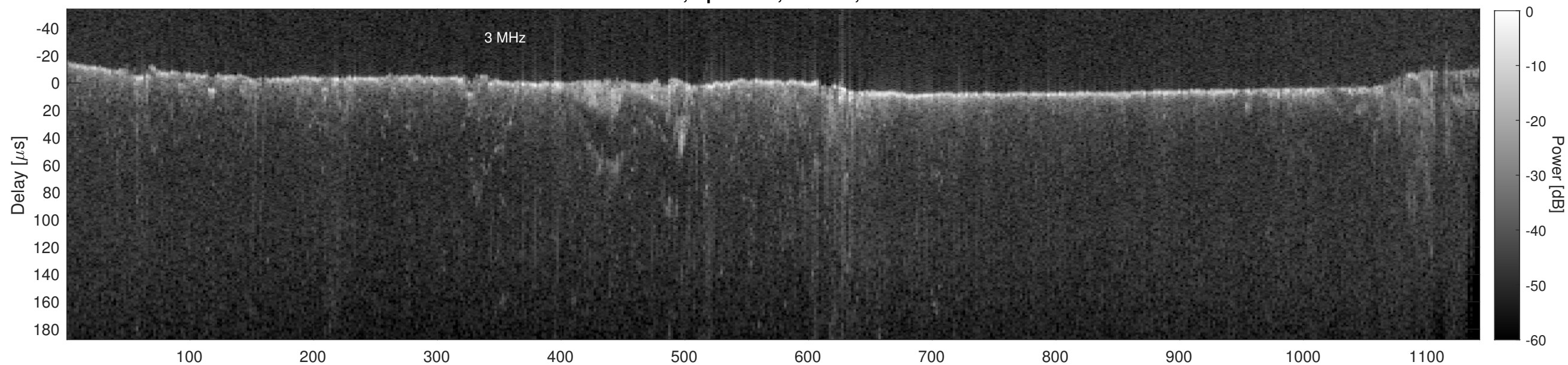
Orbit 3881, Cluttergram
