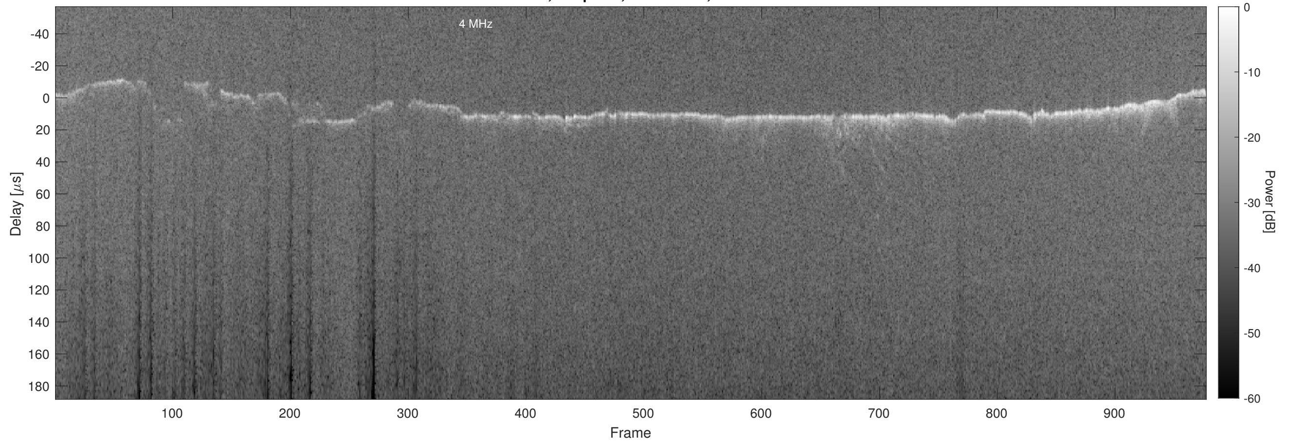
Orbit 3885, Chapman, No Window, Channel 2
