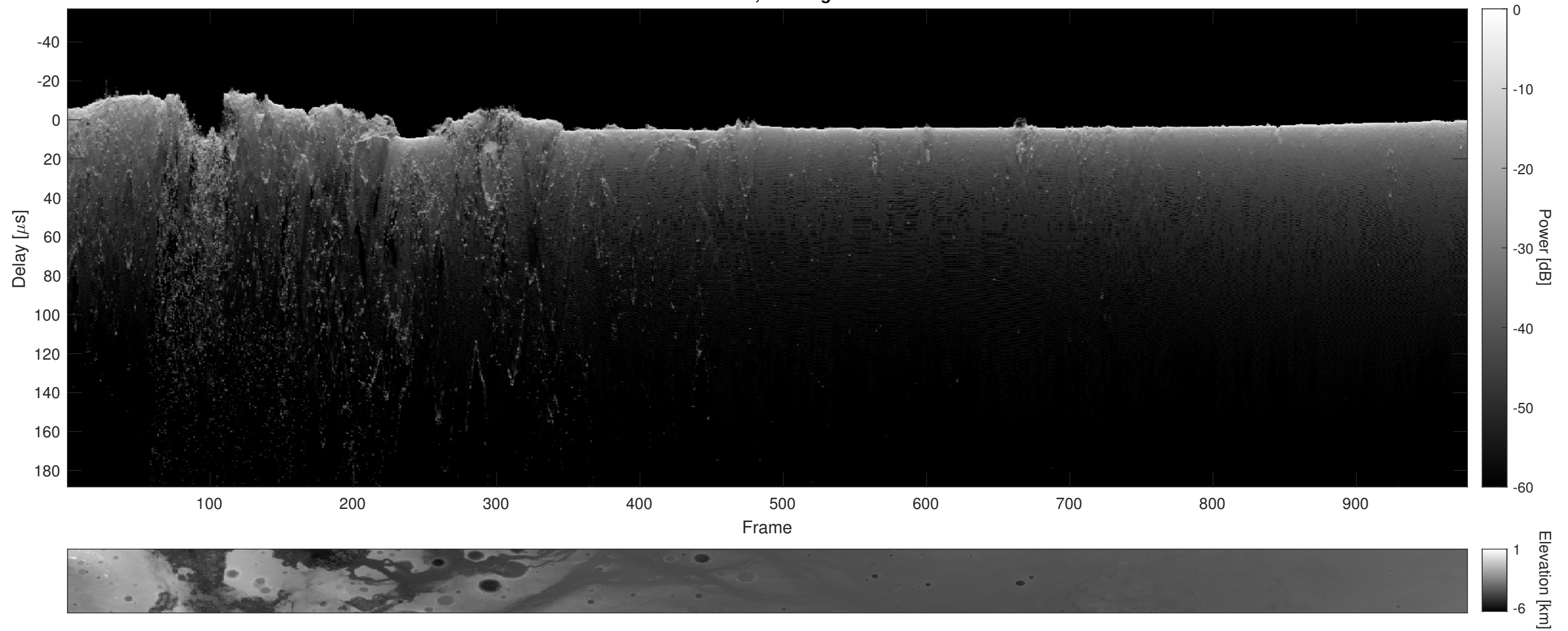
Orbit 3885, Cluttergram
