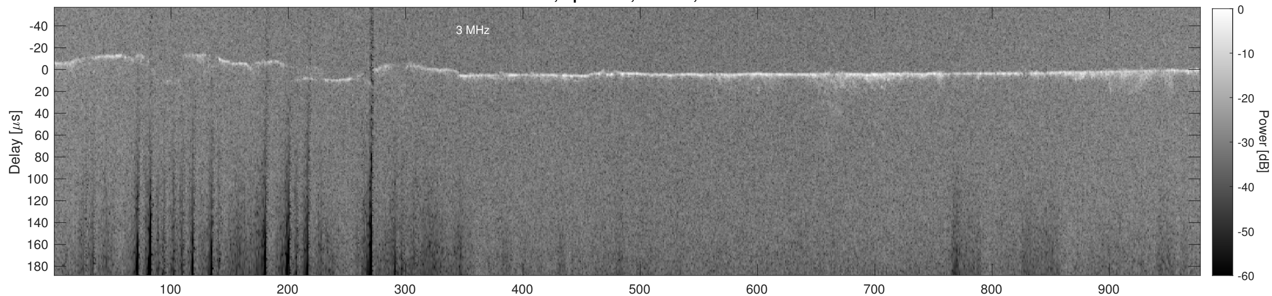
Orbit 3885, Cluttergram
