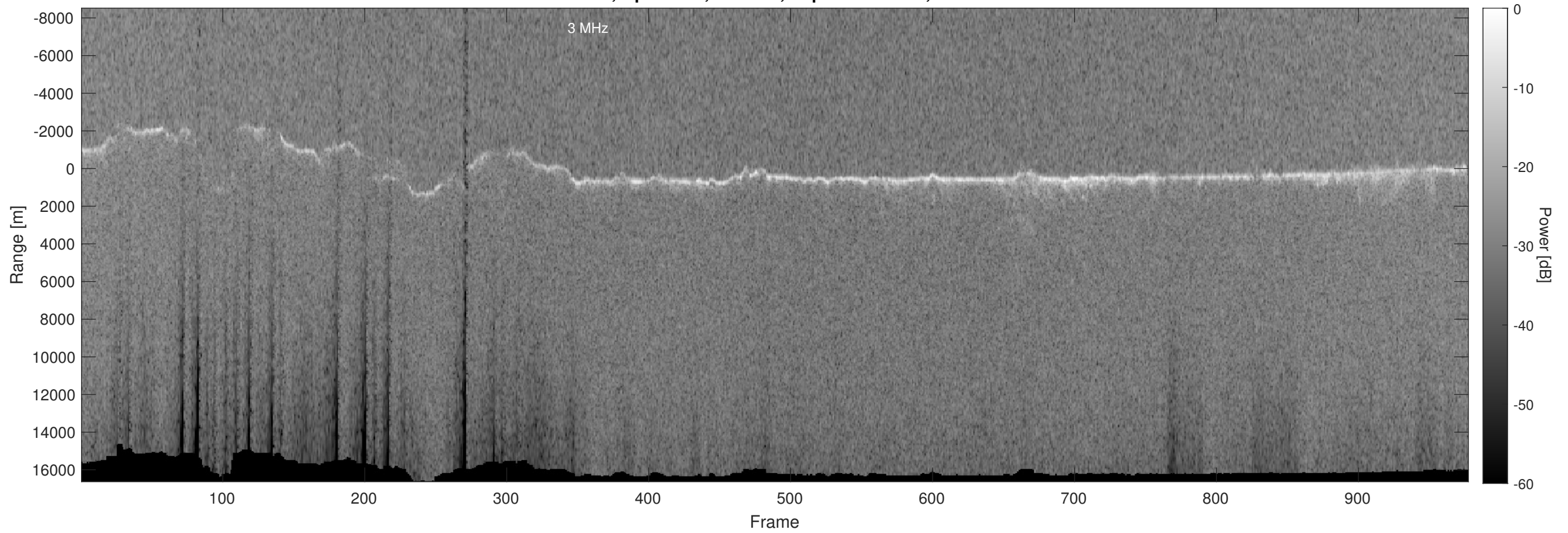
Orbit 3885, Optimized, Window, Depth-Corrected, Channel 2
