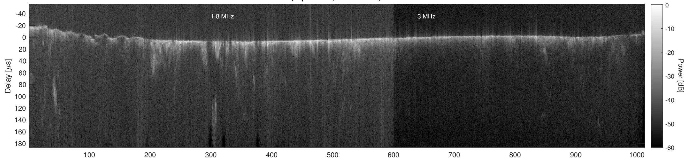
Orbit 3890, Cluttergram
