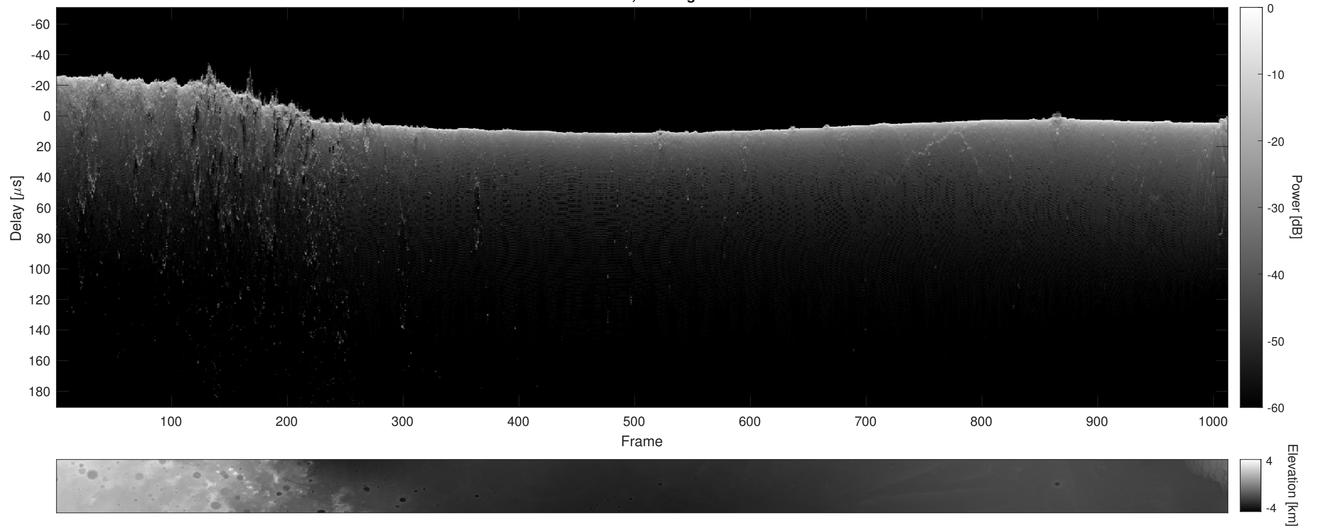
Orbit 3891, Cluttergram
