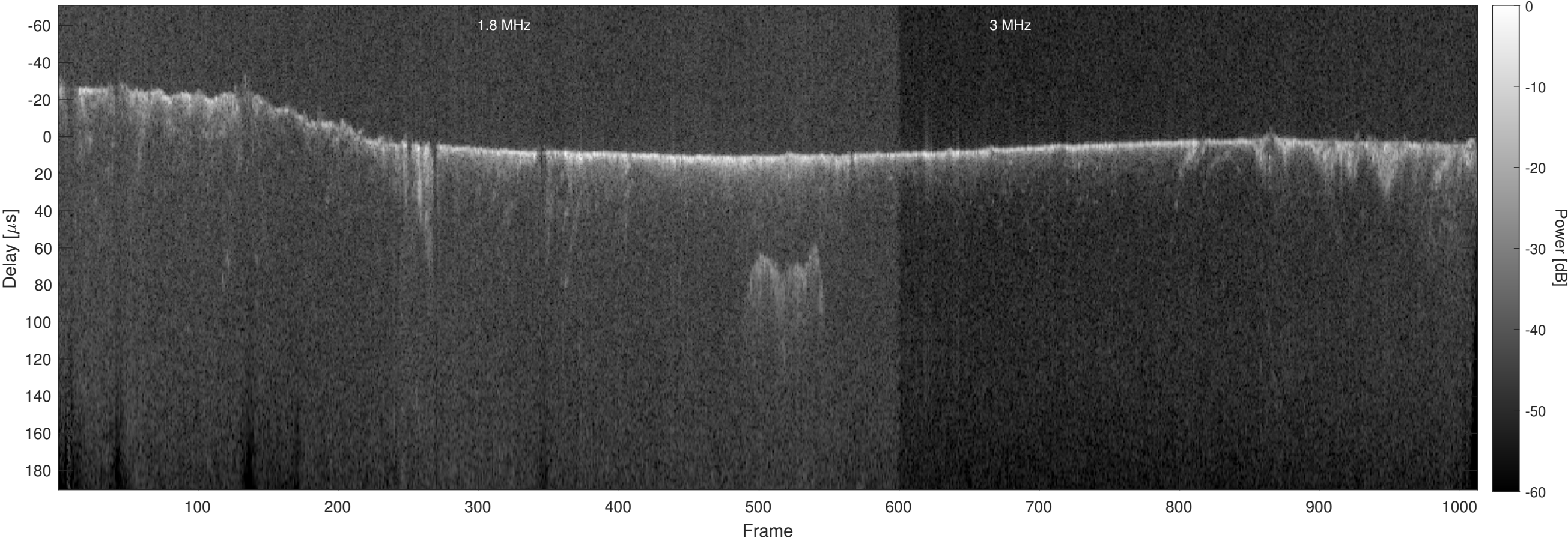
Orbit 3891, Optimized, Window, Channel 2
