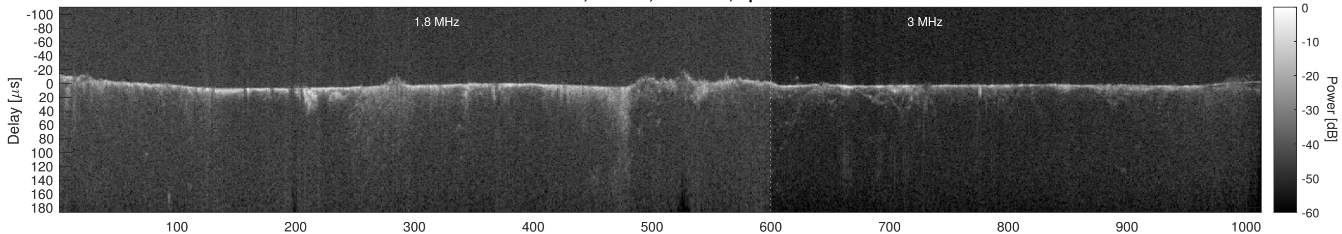
Orbit 3894, Cluttergram
