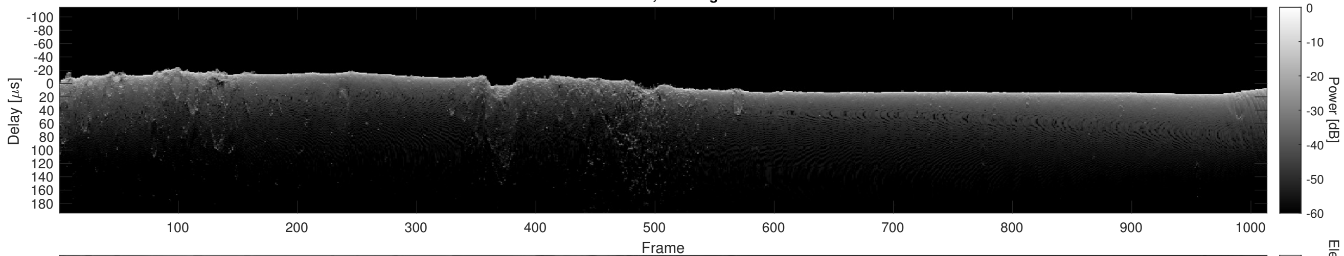
Orbit 3895, Cluttergram
