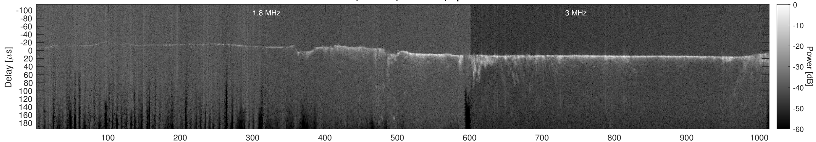
Orbit 3895, Cluttergram
