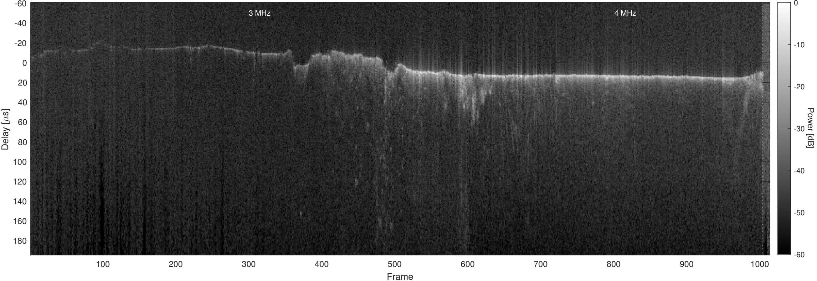
Orbit 3895, Optimized, No Window, Channel 2
