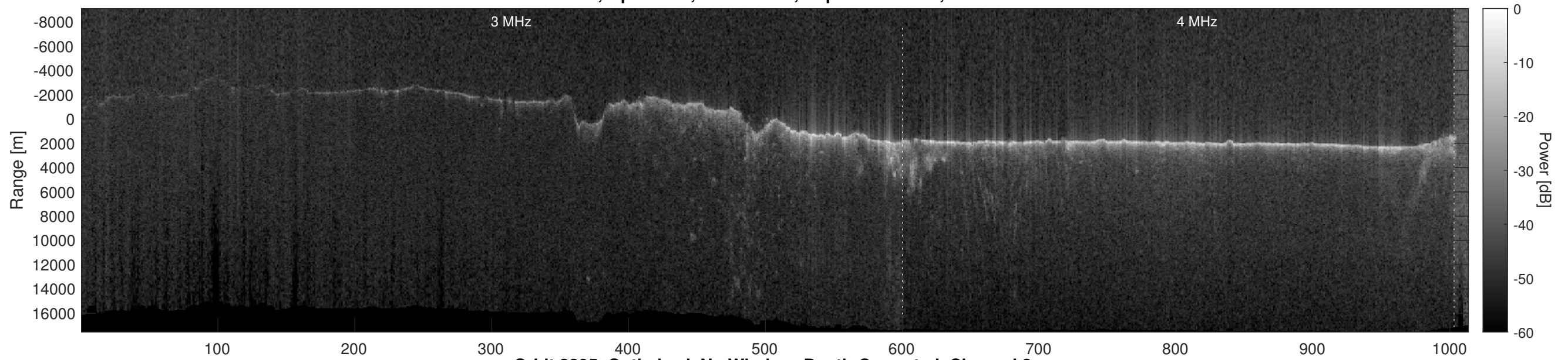
Orbit 3895, Optimized, No Window, Depth-Corrected, Channel 2
