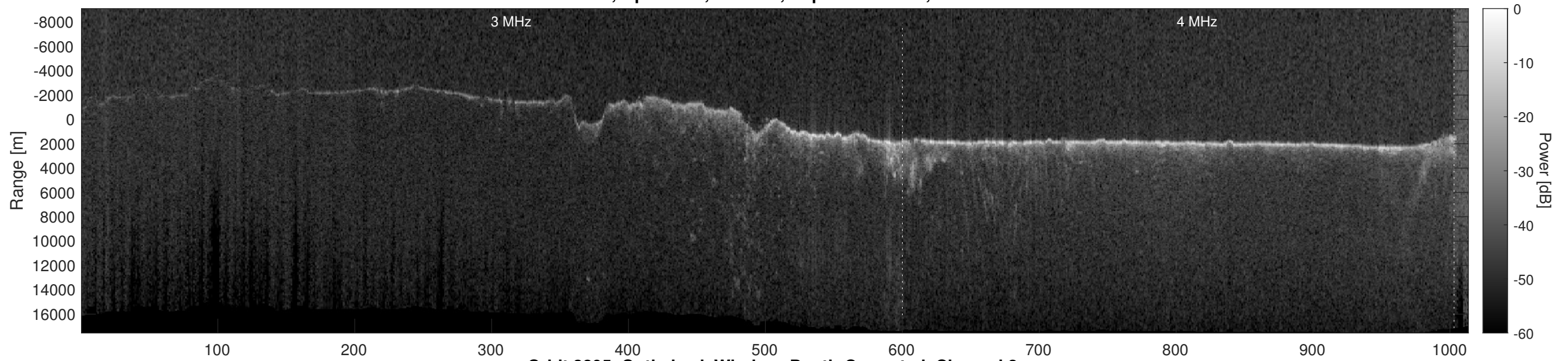
Orbit 3895, Optimized, Window, Depth-Corrected, Channel 2
