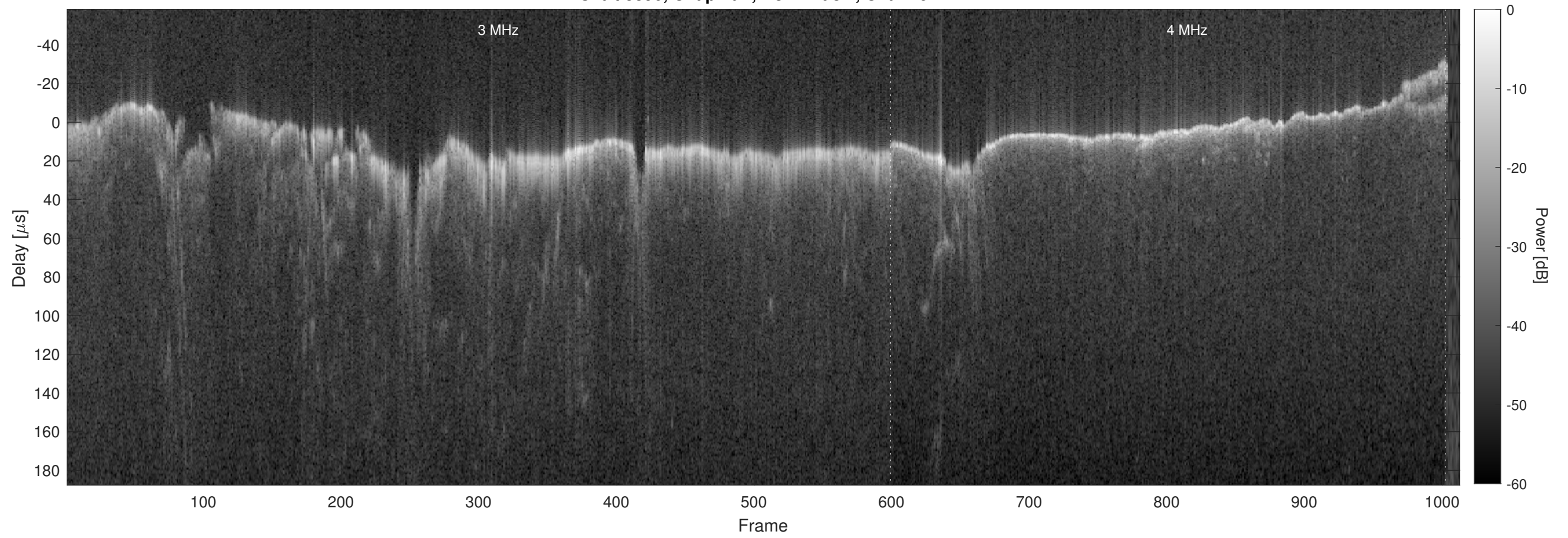
Orbit 3896, Chapman, No Window, Channel 2
