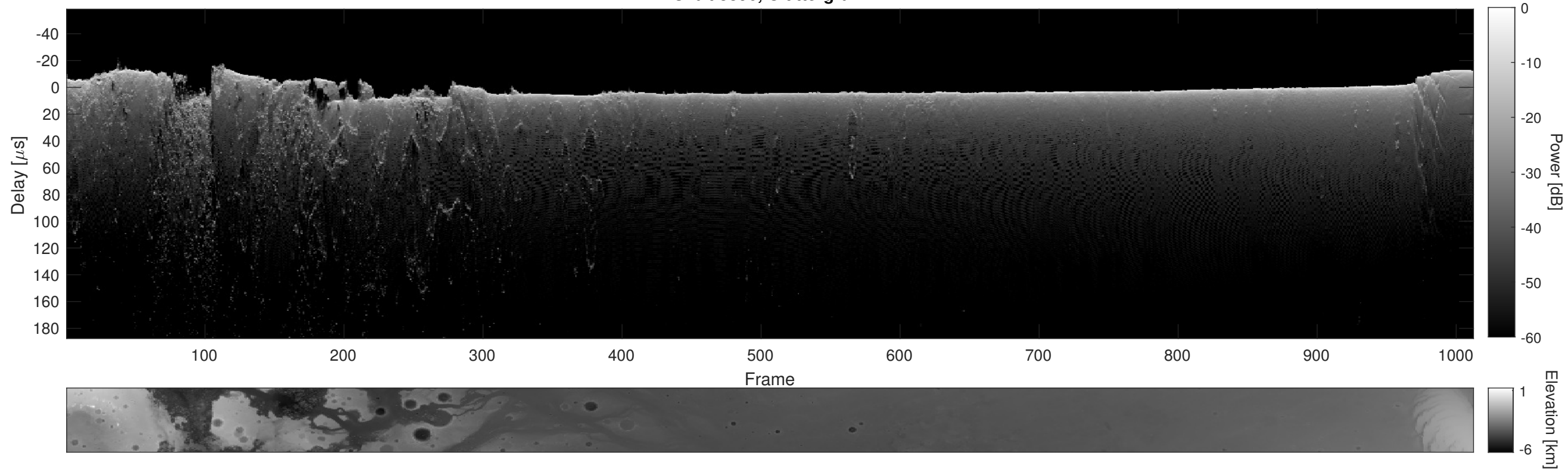
Orbit 3896, Cluttergram
