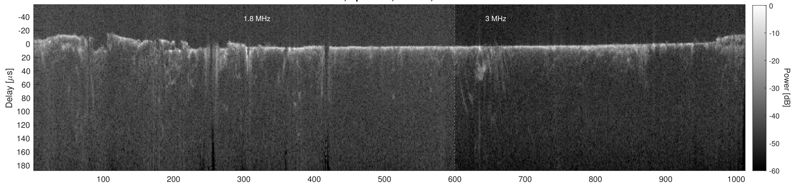
Orbit 3896, Cluttergram
