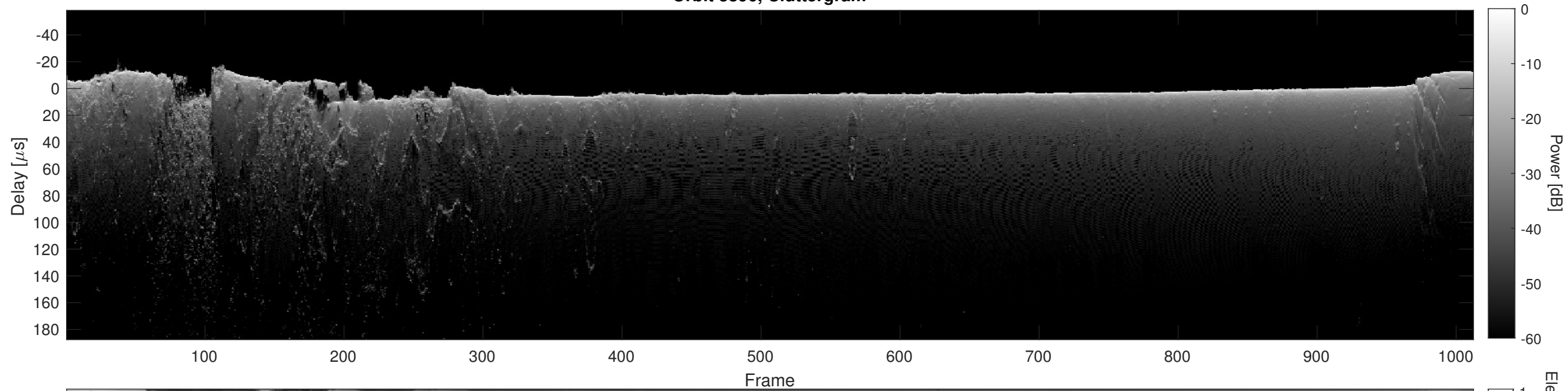
Orbit 3896, Cluttergram
